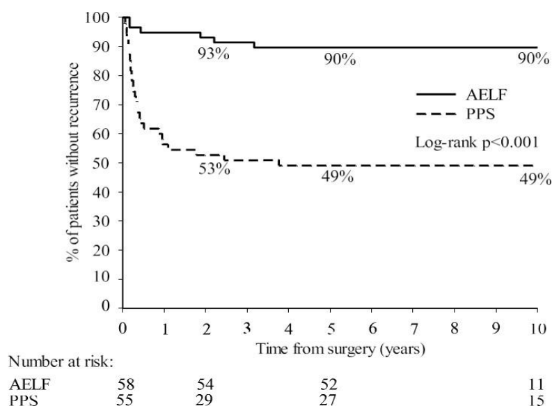
Figure 3: Kaplan–Meier curves
